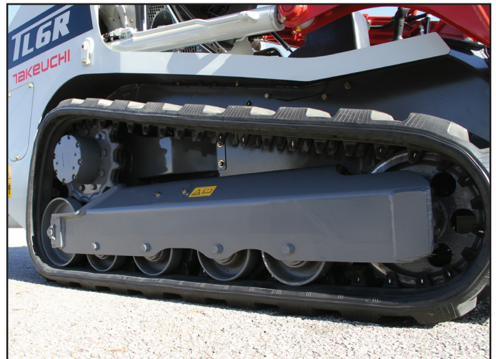
Integrated Undercarriage
