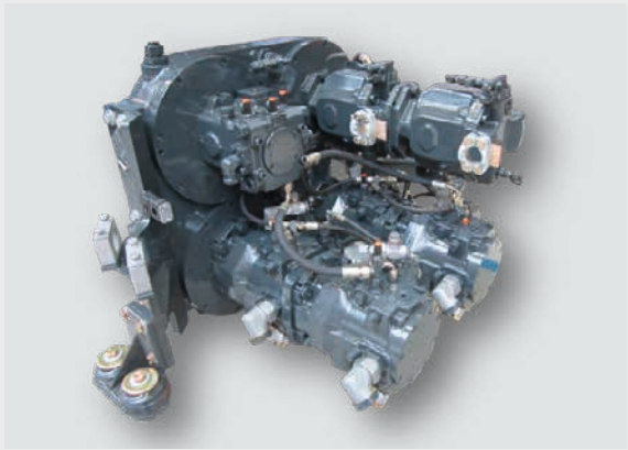
Hydraulic Quad Pump Drive with load limit control for best performance.
